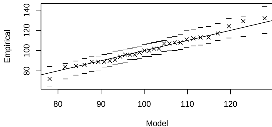
Quantile Plot
