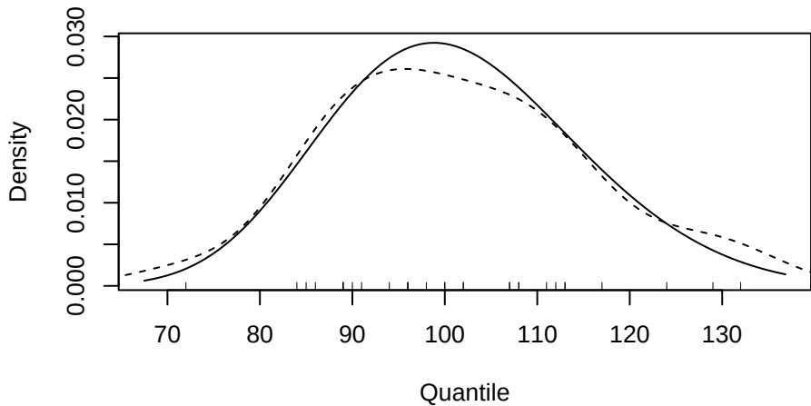
Density Plot
