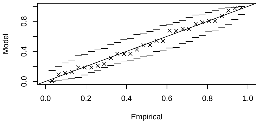
Probability Plot
